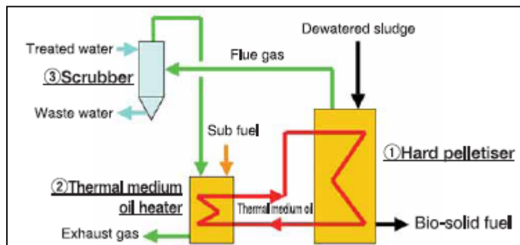
Fig.2 Flow Outline
