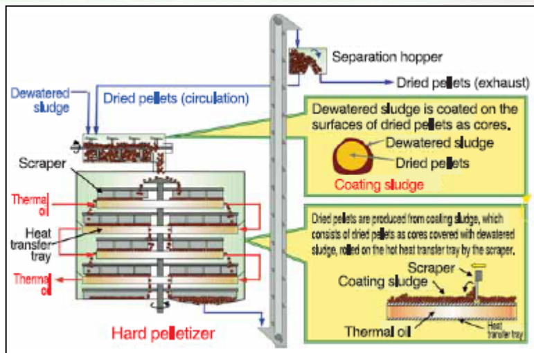
Fig.3 Principle of Drying & Hard-Pelletizing
