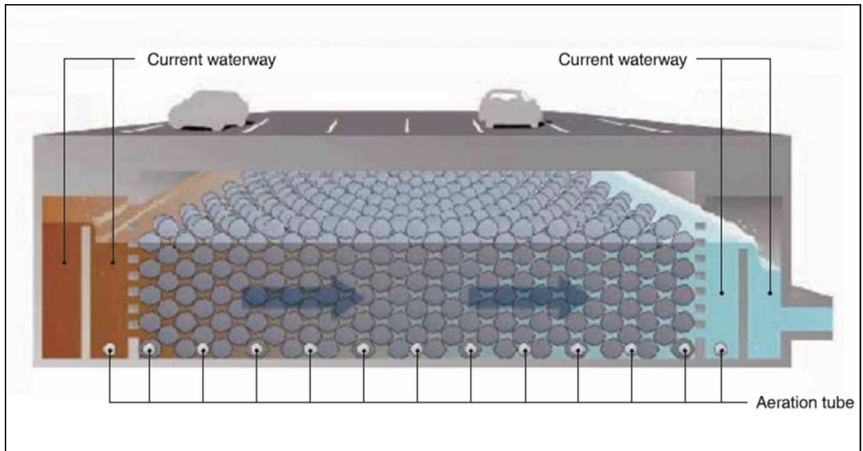
Facility overview
